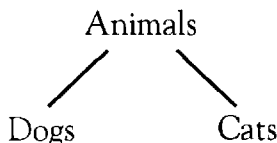
FIG. 1.1. Hierarchical classification.
