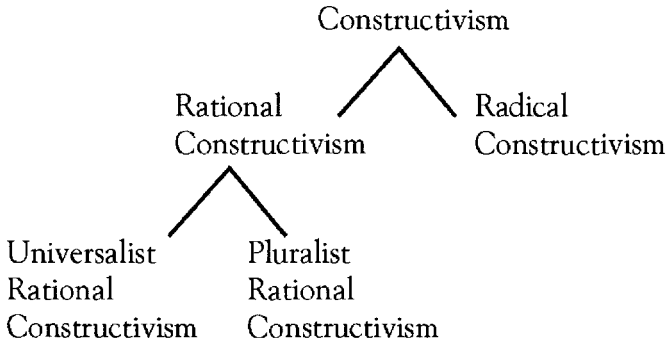
FIG. 11.2. Constructivist metatheories.
